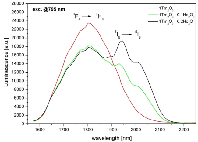
Fig. 2. Luminescence spectra for glasses doped with \text{Tm}^{3+} and \text{Tm}^{3+}/\text{Ho}^{3+} ions
