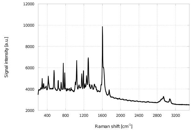
Fig. 5. Raman spectrum of Polopiryna S measured at excitation laser wavelength 785 nm having optical output power 300 mW and acquisition time of 40 s; the CCD of 1024-pixel working at temperature equal to -15^{\circ}\text{C} was applied
