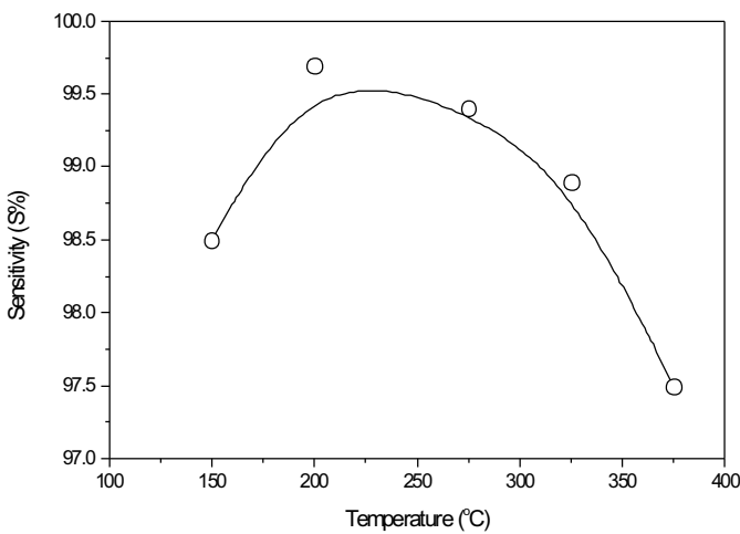
Fig. 5. Variation of percent sensitivity with sensor operating temperature for 1 vol% H 2 in air
