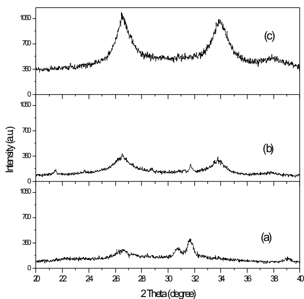
Fig. 1. XRD pattern of (a) as-deposited SnS; (b) heat treated SnS (300°C, 1 hr.); (c) heat treated SnS (400°C, 1 hr.) leading to complete conversion to \text{SnO}_2
