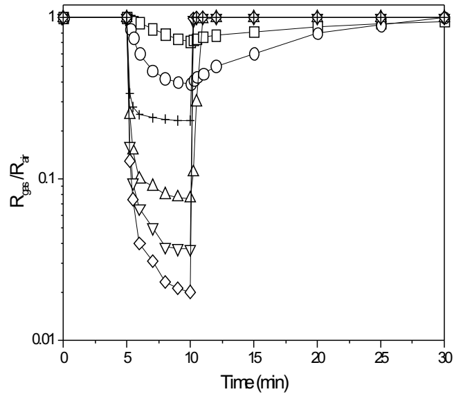
Fig. 6. Response and recovery characteristics of Pd sensitized SnO 2 film for different operating temperatures for 1.6 vol% LPG in air: 100°C (□), 200°C (○), 300°C (▽), 325°C (◇), 375°C (△) and 425°C (+)
