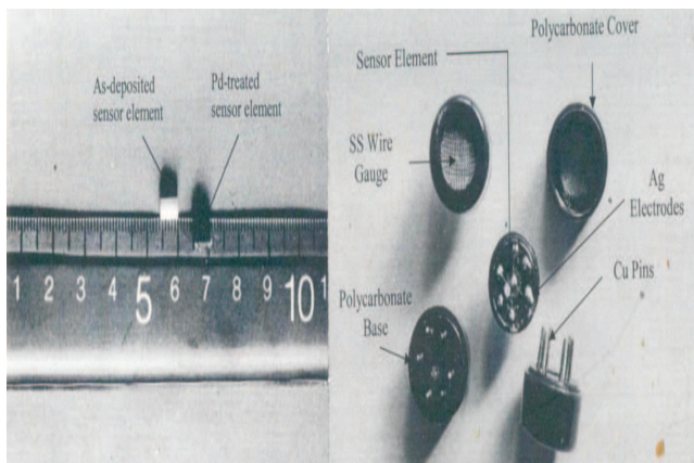
Fig. 3. As-deposited and Pd-treated sensor element on glass tube and sensor assembly housed inside a polycarbonate casing
