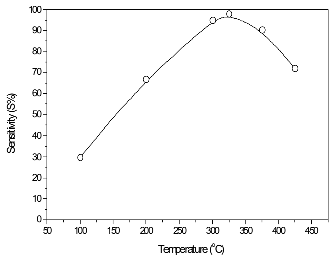
Fig. 7. Variation of percent sensitivity with sensor operating temperature for 1.6 vol% LPG in air
