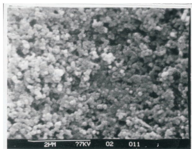
Fig. 2. SEM of \text{SnO}_2 film (thickness \sim 0.6 \mu\text{m} )
