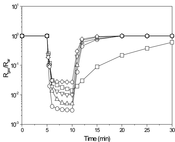
Fig. 4. Sensing and recovery characteristics of Pd sensitized SnO 2 film for different temperature in presence of 1 vol% H 2 in air: (□) 150°C, (○) 210°C, (△) 275°C, (▽) 325°C and (◇) 375°C
