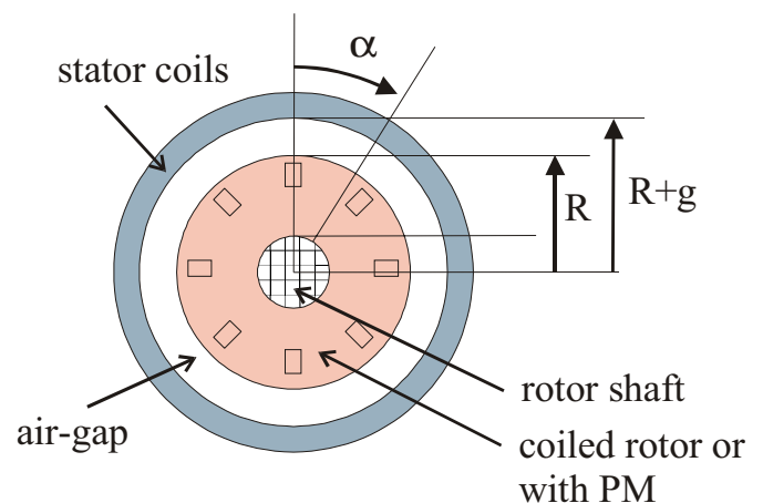
Fig. 6. Synchronous cylindrical motor model
