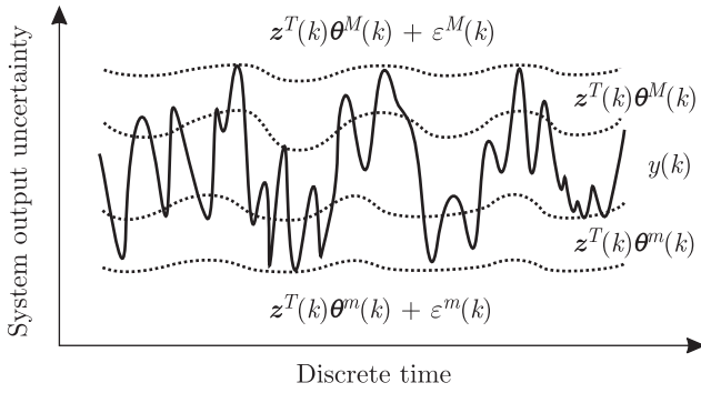
Fig. 8. System output uncertainty for the error-free regressor
