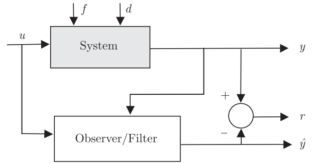
Fig. 3. Observer-based residual generator
