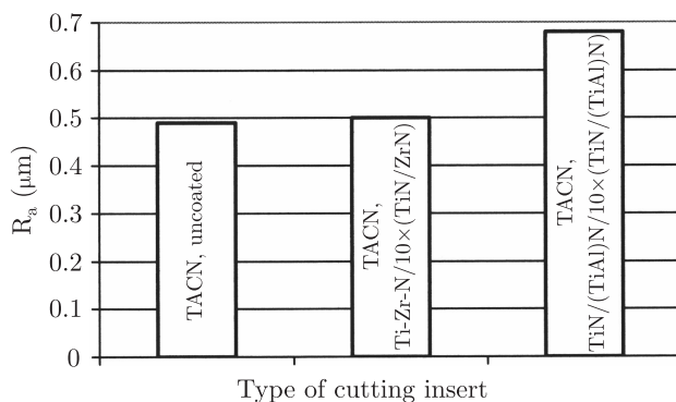
Fig. 6. Average values of roughness parameter R_a of the rollers machined with the TACN grade ceramic cutting inserts, coated and uncoated
