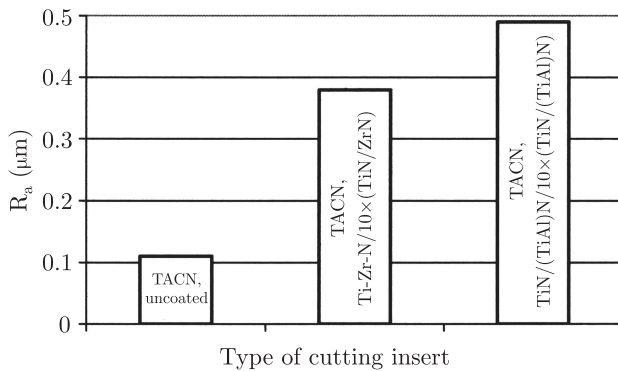
Fig. 4. Average values of roughness parameter R_a of the surfaces of TACN grade ceramic cutting inserts, coated and uncoated
