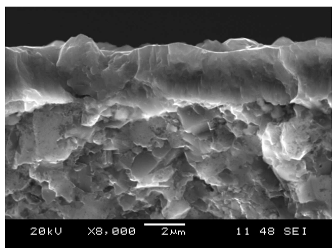
Fig. 3. A SEM micrograph showing the fractured TiN coating deposited on the TW2 grade ceramic inserts
