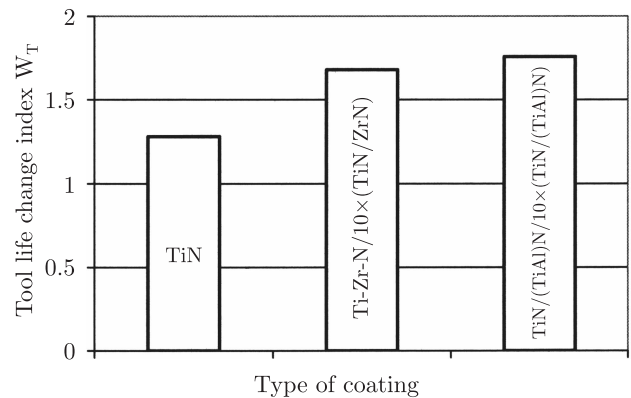
Fig. 5. Tool life change indices W_T of the coatings deposited on the TW2 grade ceramic cutting inserts
