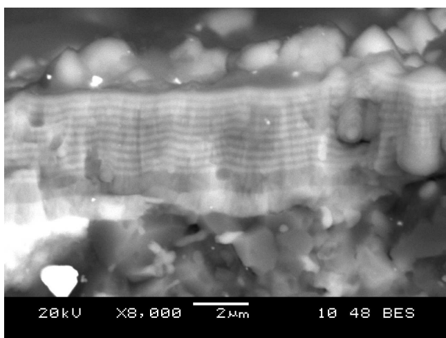
Fig. 2. A SEM micrograph showing the fractured multilayer TiN/(TiAl)N/ 10× (TiN/(TiAl)N) coating deposited on the TACN grade ceramic cutting insert
