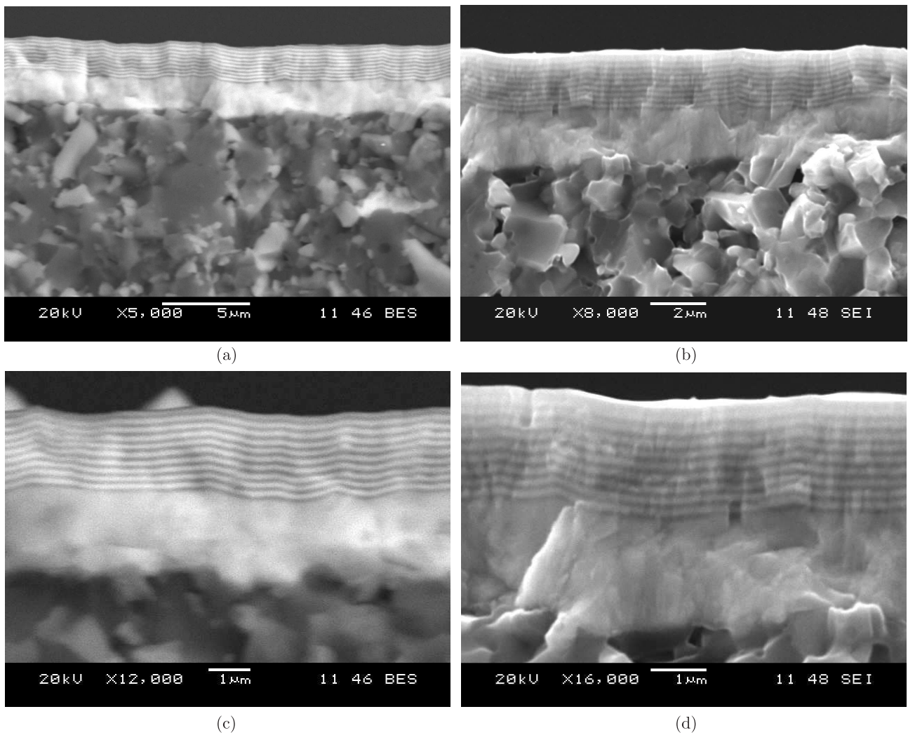
Fig. 1. SEM micrographs showing the fractured multilayer Ti-Zr-N/ 10× (TiN/ZrN) coating deposited on TACN grade ceramic cutting insert at different magnifications and types of electron image: 5000×, BES (a), 8000×, SEI (b), 12000×, BES (c) oraz 16000×, SEI (d)
