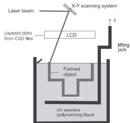
Fig. 4. Microstereolithography. The layered data from CAD successively displayed on the liquid crystal display serve as masks for the laser beam; the product (composed of ceramic powder with binder) is formed in a liquid polymerising under the action of laser radiation
