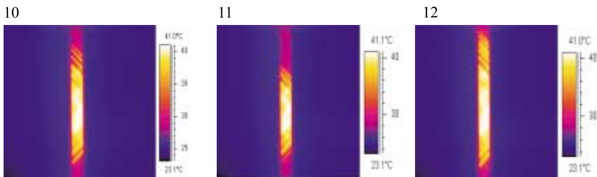
Fig. 5. Temperature distribution of TiNi SMA subjected to stress induced phase transformation during loading (martensitic transition). The numbers above the thermograms correspond to the proper points of the stress-strain curve shown in Fig. 2
